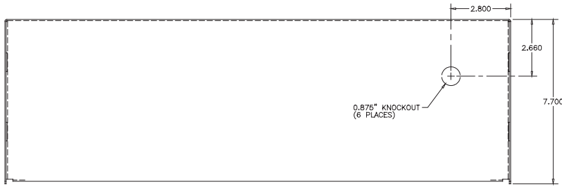
TOP VIEW
